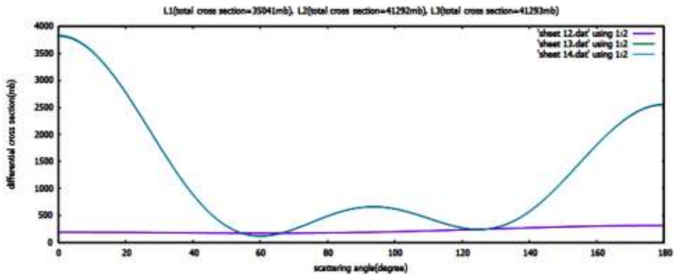
Figure 1: Graph of differential and total cross section against scattering angle with energy E_1=0.9217\text{MeV} and angular momentum ( l=1, 2 and 3 ) for ^{56}\text{Fe} isotope.
