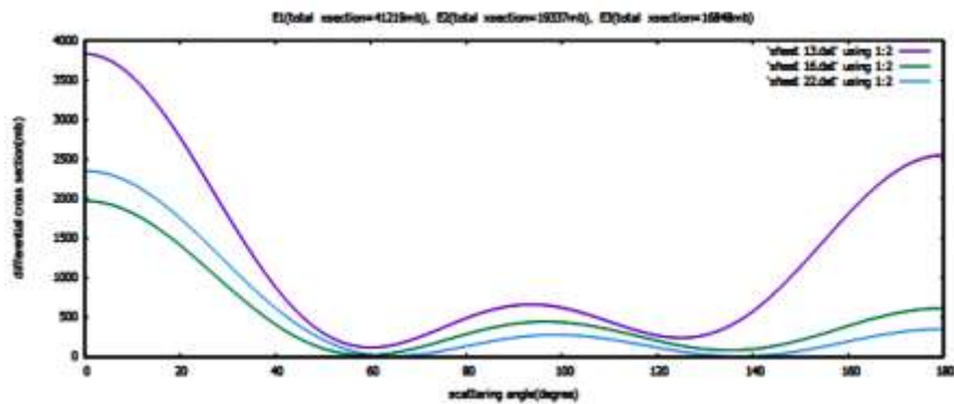
Figure 3: Graph of differential and total cross section against scattering angle with the angular momentum l=2 and Energies: E_3=1.6385\text{MeV} , E_2=3.7001\text{MeV} , E_1=14.747\text{MeV} for ^{56}\text{Fe} isotope
