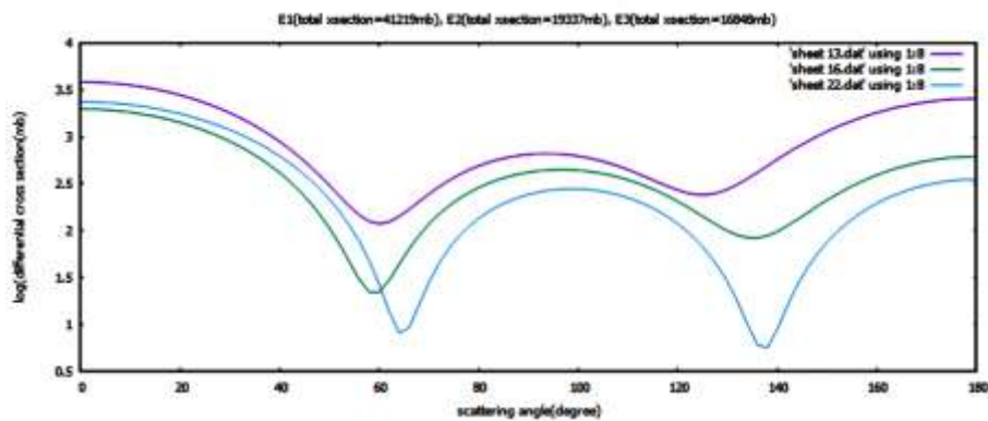
Figure 4: Graph of log of differential cross section against scattering angle with the angular momentum l=2 and Energies: E_3=1.6385\text{MeV} , E_2=3.7001\text{MeV} , E_1=14.747\text{MeV} for ^{56}\text{Fe} isotope.
