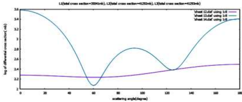
Figure 2: Graph of log of differential cross section against scattering angle with energy E_1=0.9217\text{MeV} and angular momentum ( l=1, 2 and 3 ) for ^{56}\text{Fe} isotope.
